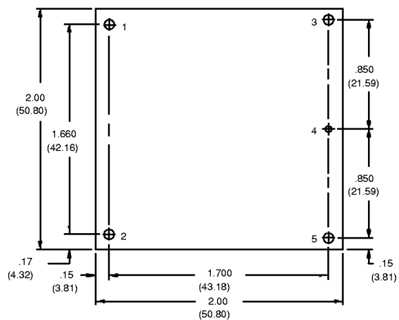
AA25E-005L-033S BOTTOM VIEW
