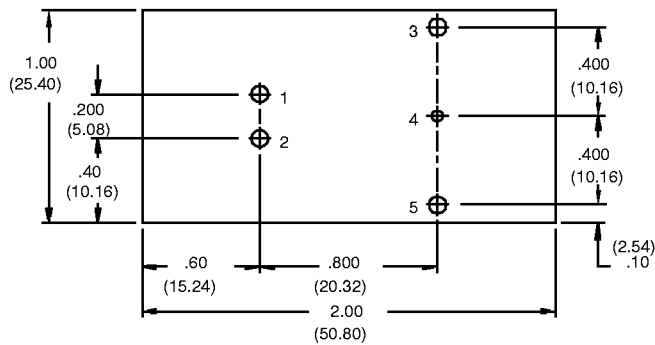
AA13A-005L-033S BOTTOM VIEW
