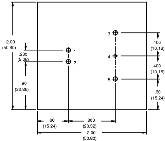
AA25D-005L-033S BOTTOM VIEW
