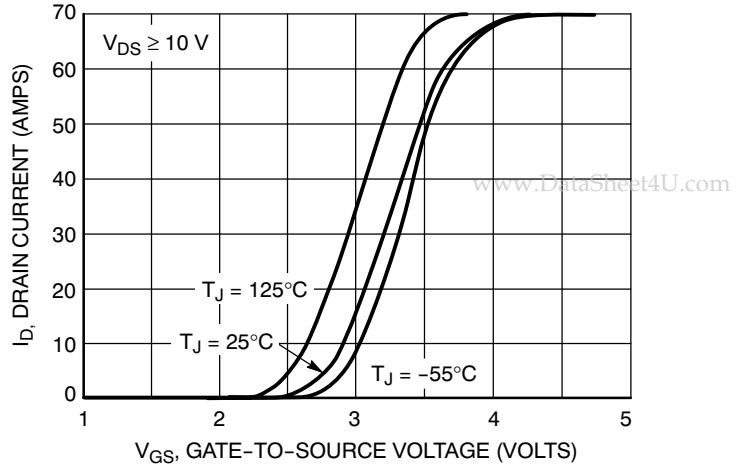
Figure 2. Transfer Characteristics
